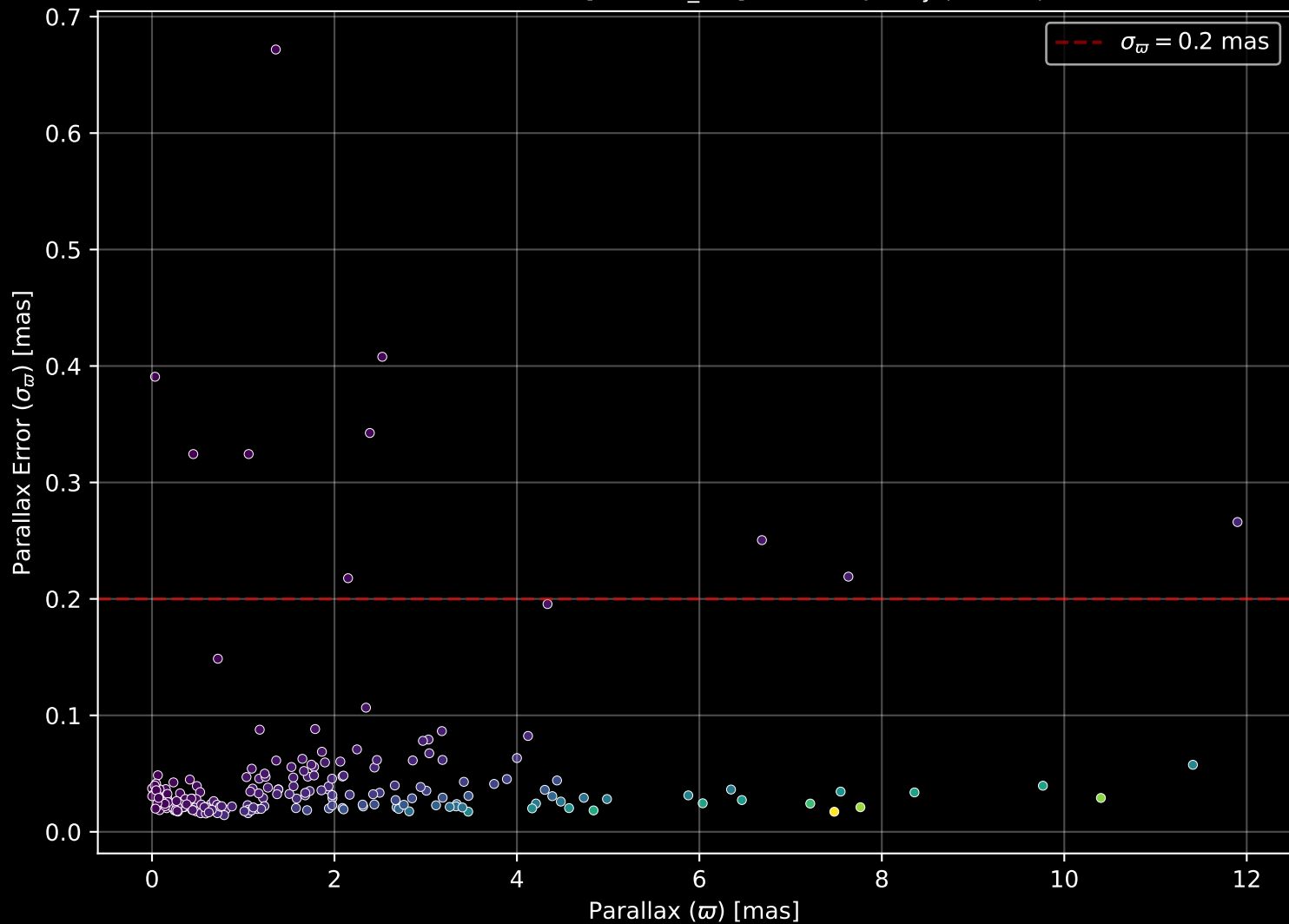
APOGEE DR17 Field: [279+61_btx] Parallax Quality (n= 203)
