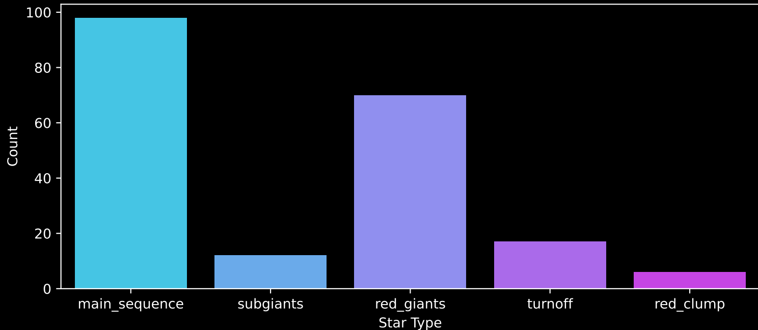
APOGEE DR17 Field: [279+61_btx] Count plot of Star Type
