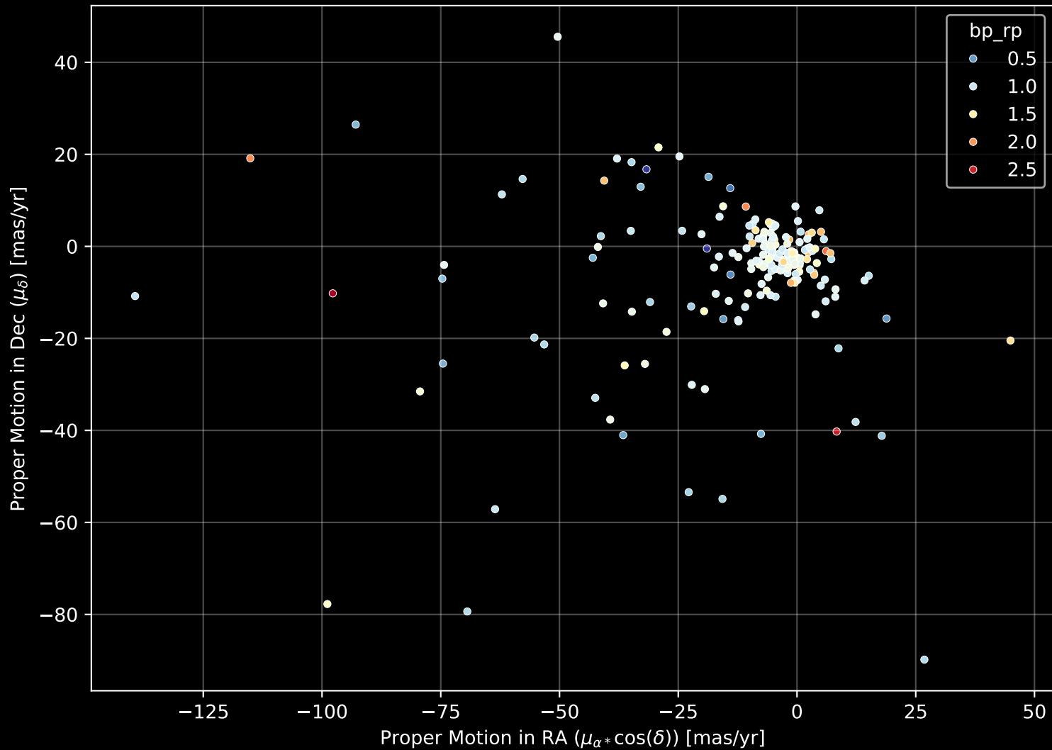
APOGEE DR17 Field: [279+61_btx] Proper Motion Diagram (n= 203)
