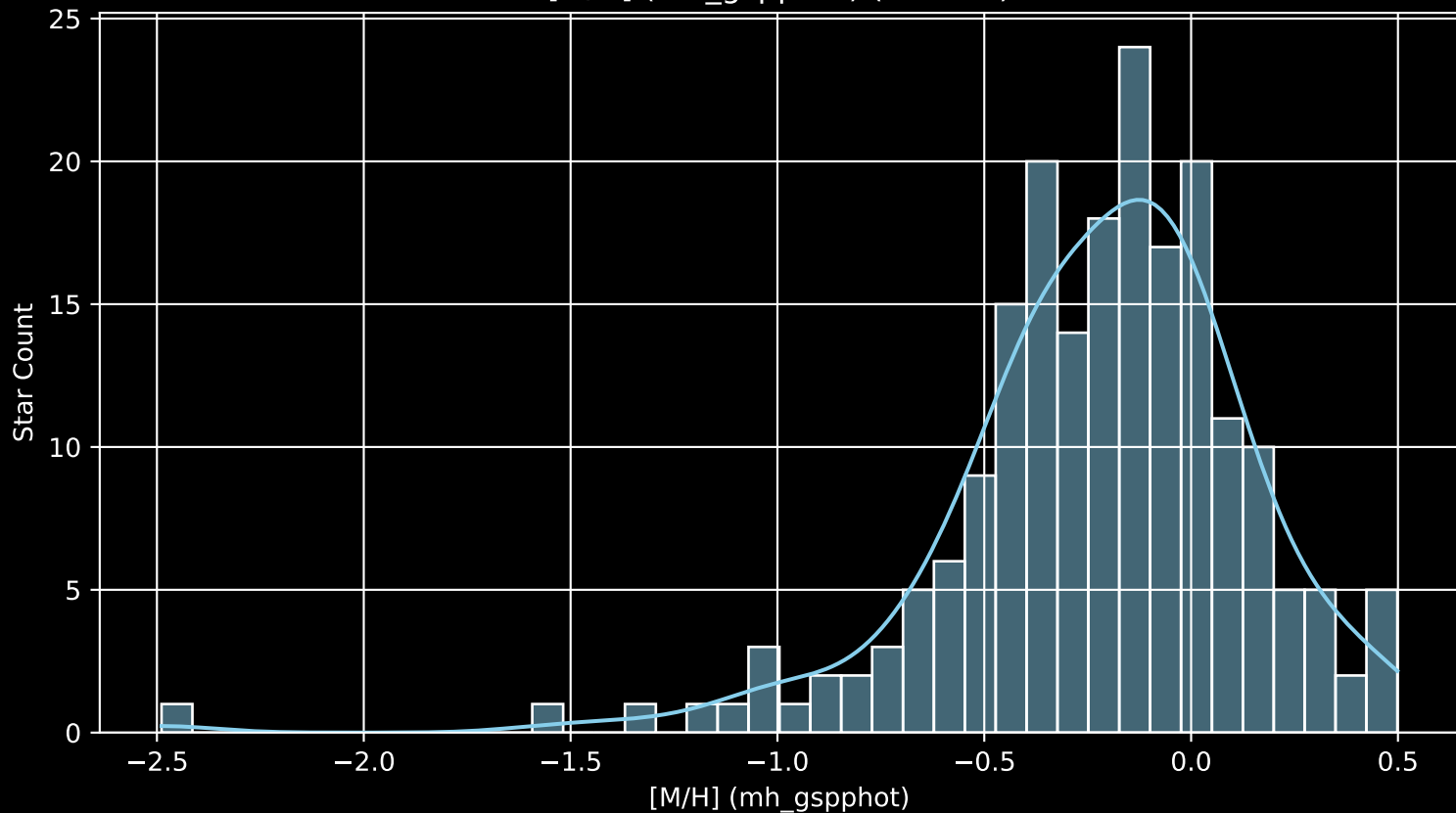
APOGEE DR17 Field: [279+61_btx [M/H] (mh_gspphot) (n= 202)
