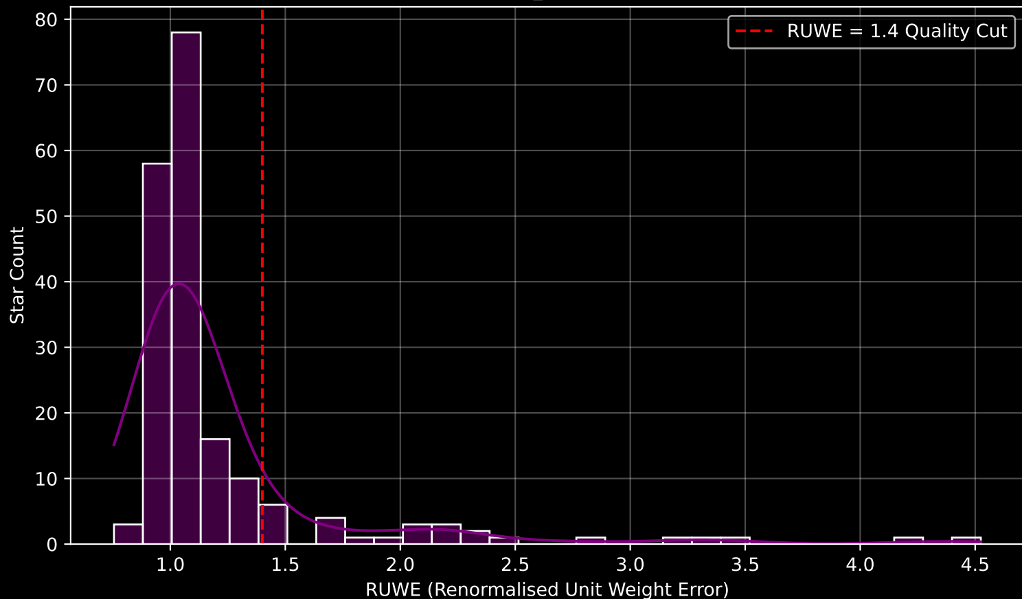
GAPOGEE DR17 Field [279+61_btx] RUWE Distribution (n= 192)
