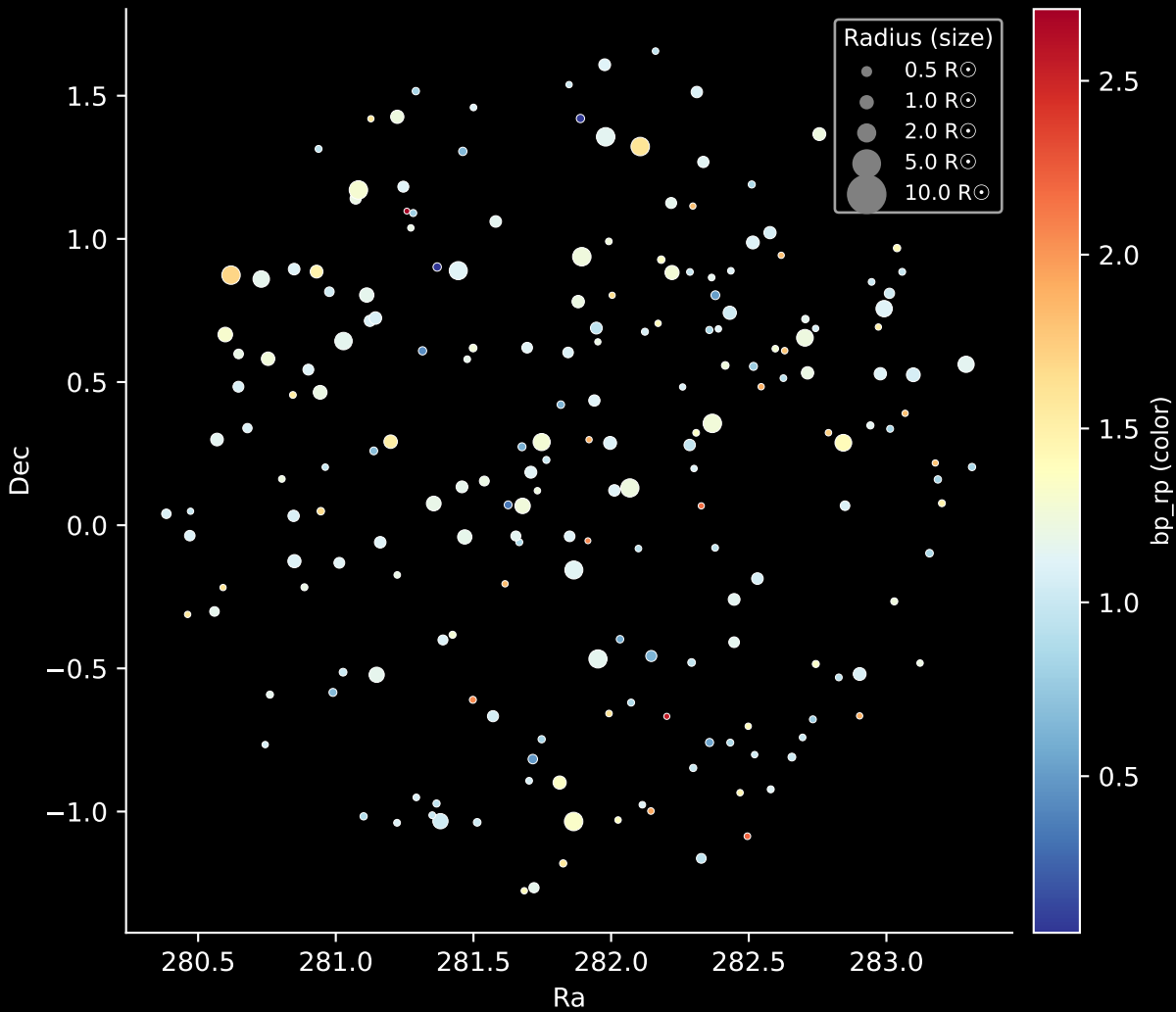
APOGEE DR17 Field: [279+61_btx] Stars: 203
